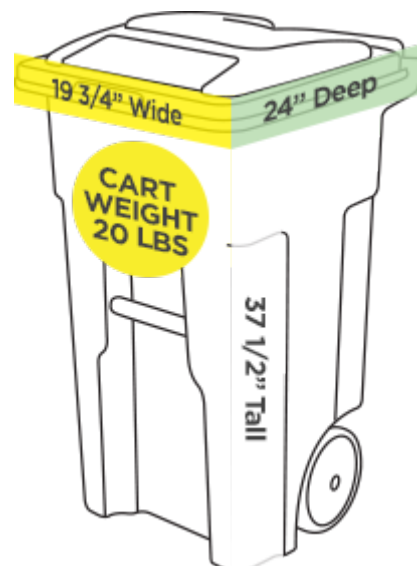
Figure 4 – 32 gallon (0.16 cy)
