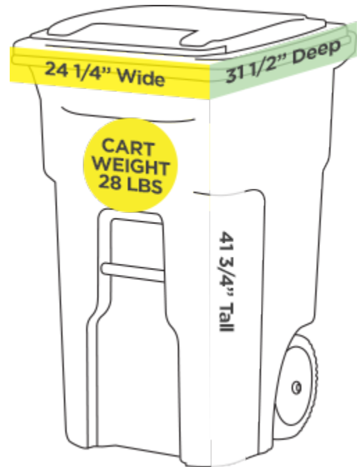
Figure 2 – 64 gallon (0.32 cy)
